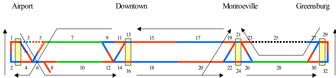
Figure 4-4: Route of switch hazards in Airport/Downtown region
