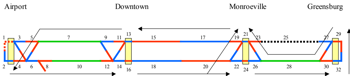
Figure 4-7: Route of segment 1 out-of-service
