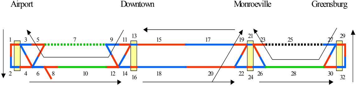
Figure 4-10: Route of segment 7 out-of-service
