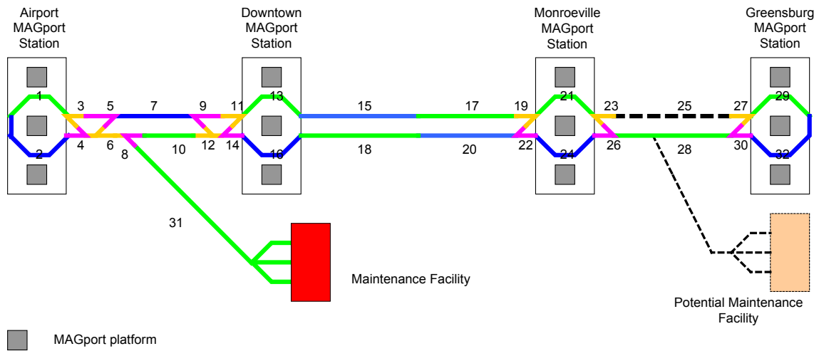
Figure 2-1: Pennsylvania Project Dual Guideway
